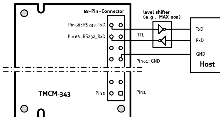
Figure 7.4: Connecting RS232
